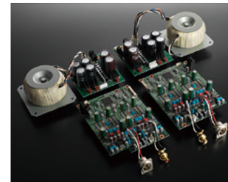
Left and right DAC circuit boards, and individual power supply units
